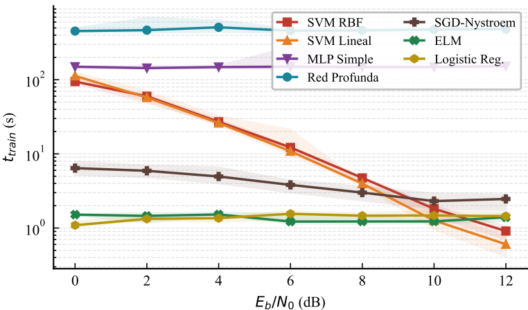
Training time vs E_b/N_0 — Median \pm IQR
